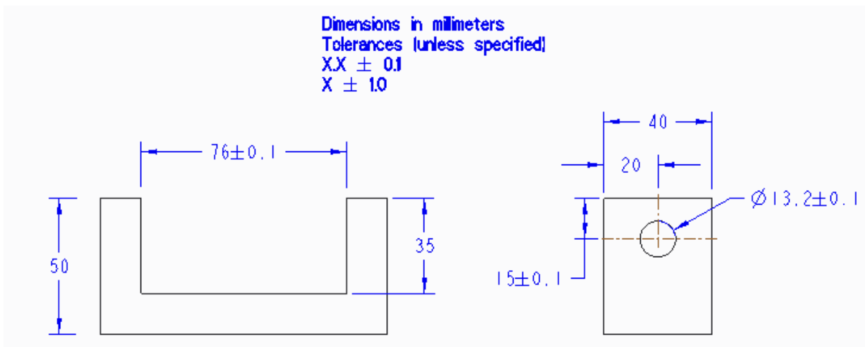
Fig.2 C blocks dimensions
