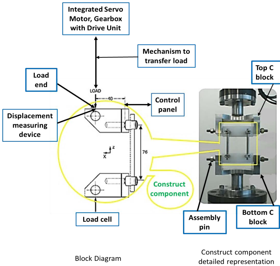
Fig.1 Fatigue test setup (Pictorial representation only)
